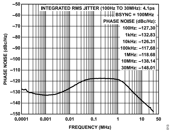
Figure 13. BSYNC Output Absolute Phase Noise, 100 MHz
