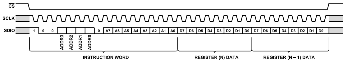
Figure 50. 3-Wire SPI Control Port Read—MSB First, Address Decrement, and Two Bytes of Data
