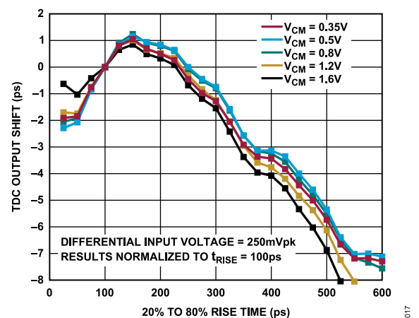
Figure 17. TDC Output Shift vs. Incoming BSYNC Time Rise for Various Common-Mode Voltages
