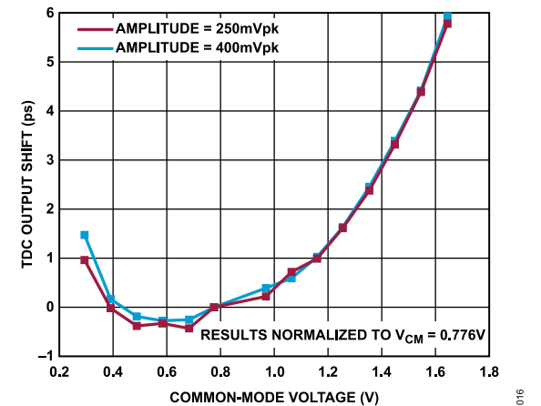
Figure 16. TDC Output Shift vs. Incoming BSYNC Common-Mode Voltage for Various Amplitudes
