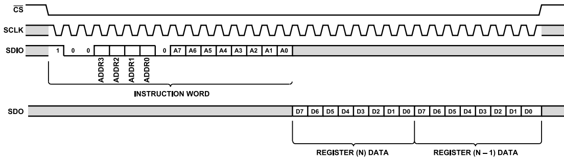
Figure 51. 4-Wire SPI Control Port Read—MSB First, Address Decrement, and Two Bytes of Data
