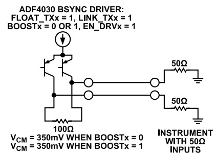
Figure 40. ADF4030 BSYNC Driver to 50 \Omega Instrument Connection
