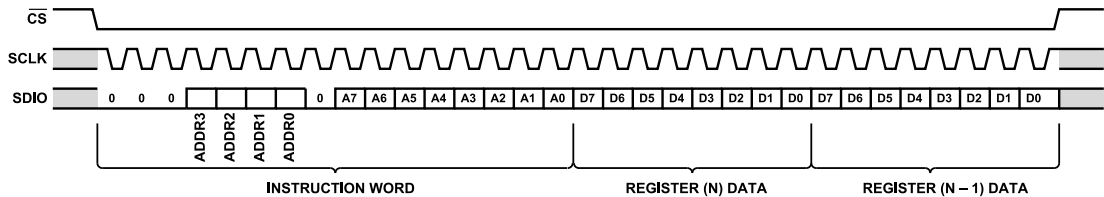
Figure 49. SPI Control Port Write—MSB First, Address Decrement, and Two Bytes of Data
