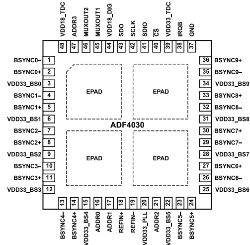
Figure 5. Pin Configuration
