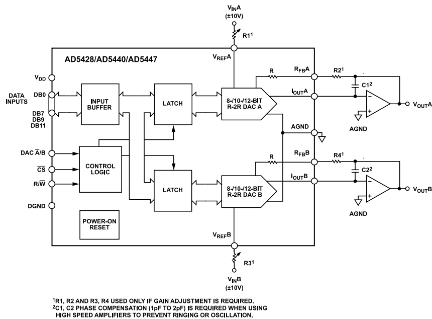
Figure 38. Unipolar Operation
