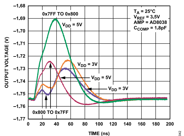
Figure 24. Midscale Transition, V_{REF} = 3.5\text{ V}
