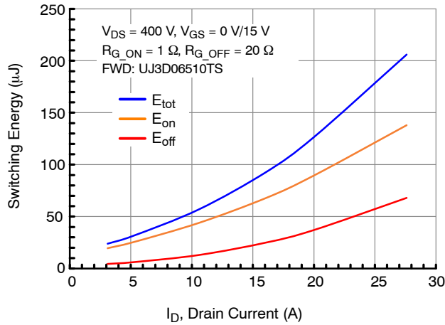
Figure 25. Clamped Inductive Switching Energy vs. Drain Current at V_{DS} = 400\text{ V} and T_J = 25\text{ °C}
