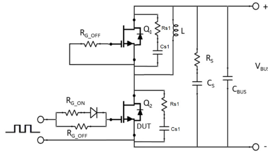
Figure 31. Schematic of the Half-Bridge Mode Switching Test Circuit with device RC Snubber ( R_{S1} = 10\ \Omega , C_{S1} = 95\ \text{nF} ) and a Bus RC Snubber ( R_S = 2.5\ \Omega , C_S = 100\ \text{nF} ).
