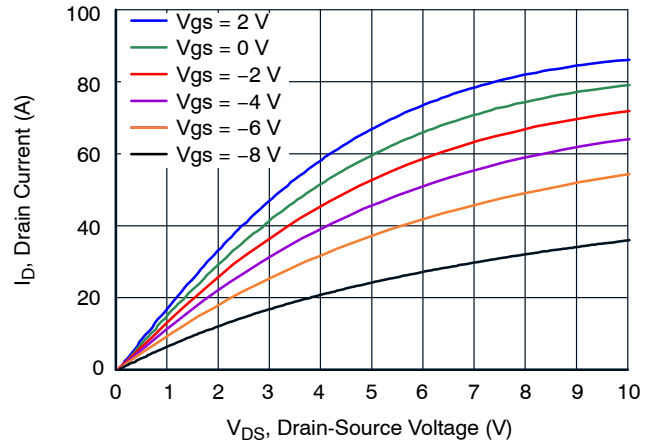
Figure 2. Typical Output Characteristics at T_J = 25^\circ\text{C}
