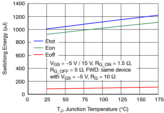
Figure 21. Clamped Inductive Switching Energy vs. Junction Temperature at V_{DS} = 400 V and I_D = 80 A
