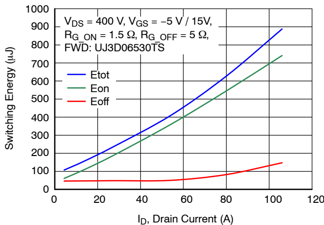
Figure 23. Clamped Inductive Switching Energy vs. Drain Current at T_J = 25 °C
