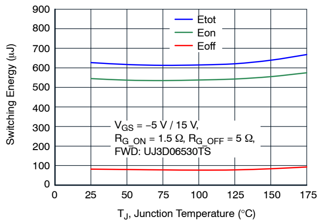
Figure 24. Clamped Inductive Switching Energy vs. Junction Temperature at V_{DS} = 400 V and I_D = 80 A
