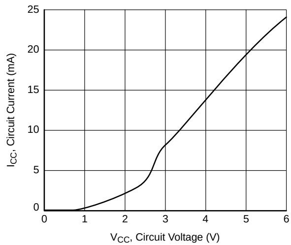
Figure 3. I_{CC} - V_{CC}
