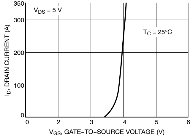
Figure 12. Transfer Characteristics
