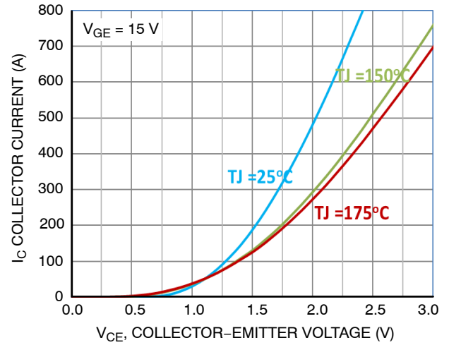
Figure 28. Saturation Voltage Characteristic
