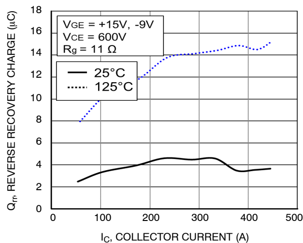
Figure 88. Typical Reverse Recovery Charge vs. I_C
