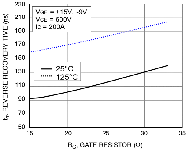
Figure 55. Typical Reverse Recovery Time vs. R_G
