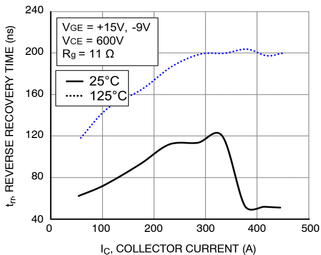
Figure 87. Typical Reverse Recovery Time vs. I_C
