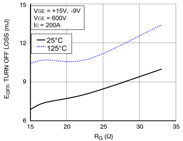
Figure 44. Typical Turn Off Loss vs. R_G
