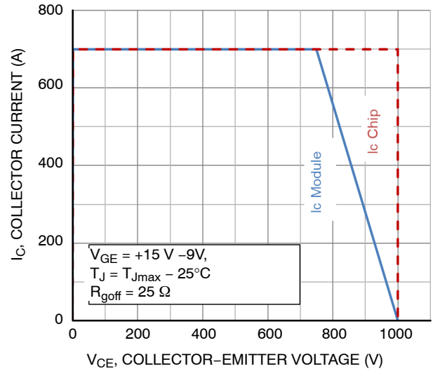
Figure 21. RBSOA
