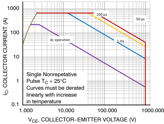
Figure 29. FBSOA
