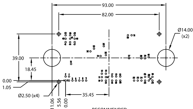
RECOMMENDED MOUNTING PATTERN
