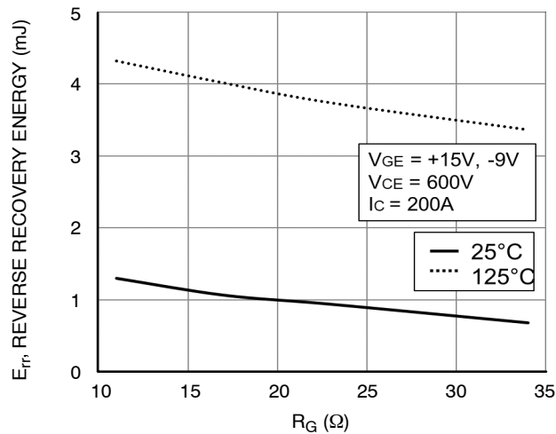
Figure 86. Typical Reverse Recovery Energy Loss vs. R_G
