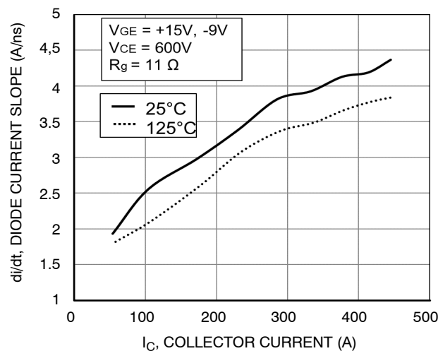
Figure 90. Typical di/dt vs. I_C
