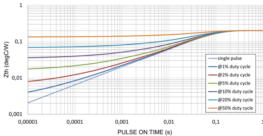
Figure 18. Transient Thermal Impedance (Neutral Point Diode Z_{thjc} )
