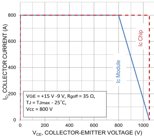
Figure 10. RBSOA (T2-T3)
