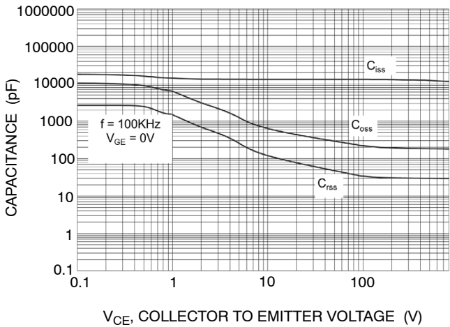
Figure 27. Capacitance Charge
