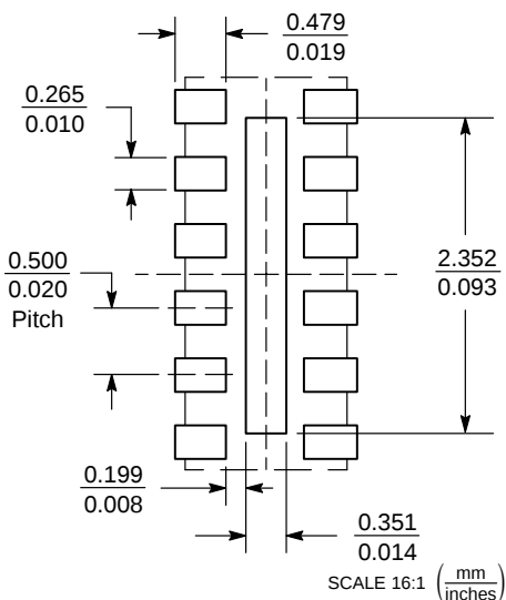
SOLDERING FOOTPRINT*
