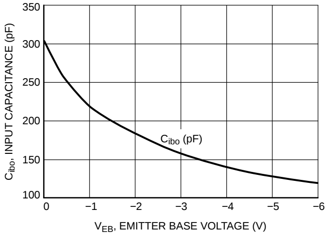
Figure 17. Input Capacitance
