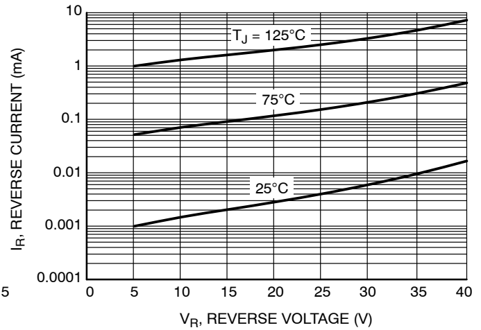
Figure 4. Leakage Current
