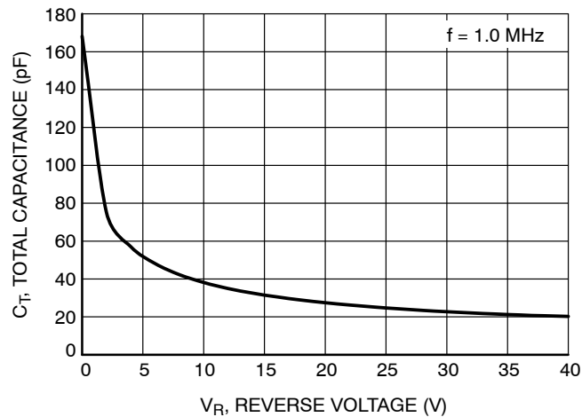
Figure 7. Total Capacitance
