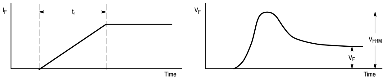
Figure 2. Peak Forward Recovery Voltage Definition
