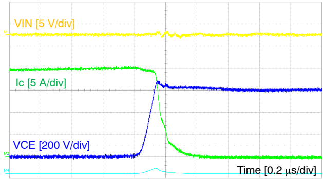
Figure 24. Turn-of Switching Waveform
