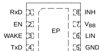
DFN8 (Top View)
