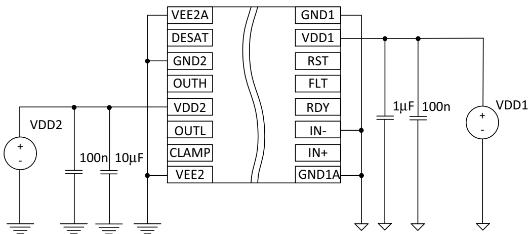
Figure 12. Unipolar Power Supply
