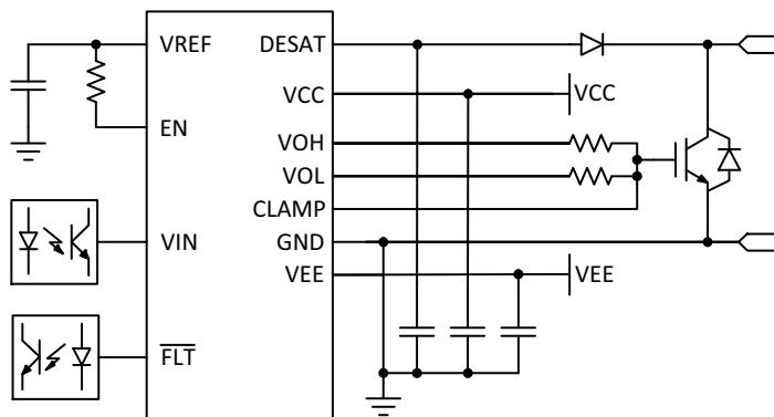
Figure 1. Simplified Application Schematic
