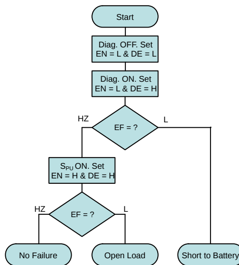
Figure 14. Flowchart for Diagnostics in OFF State
