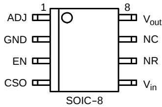
Figure 3. Pin Connections (Top View)
