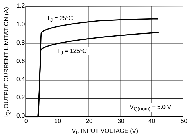
Figure 12. Output Current I_Q vs. Input Voltage V_I
