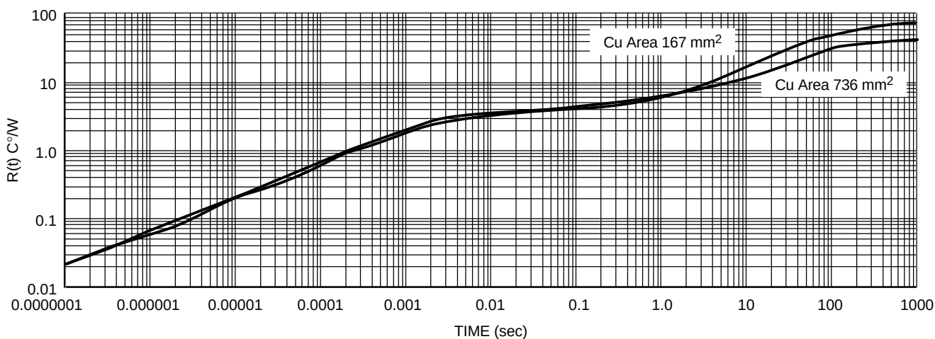
Figure 31. Single-Pulse Heating Curves, D²PAK 5-Lead
