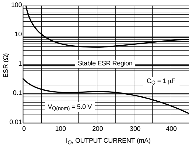
Figure 4. Output Stability with Output Capacitor ESR
