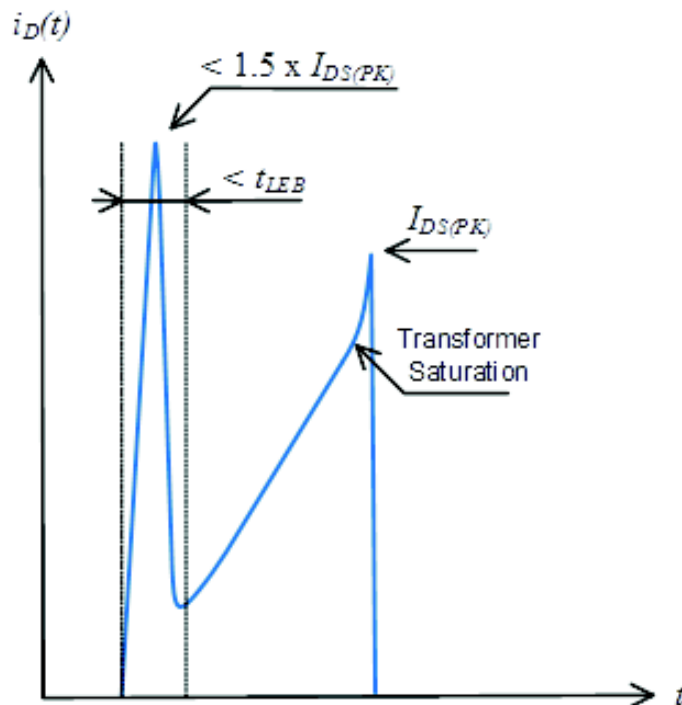
Figure 3. Spike Limits
