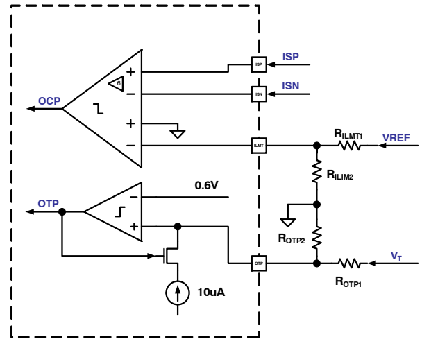
(2) OTP Configuration 2
