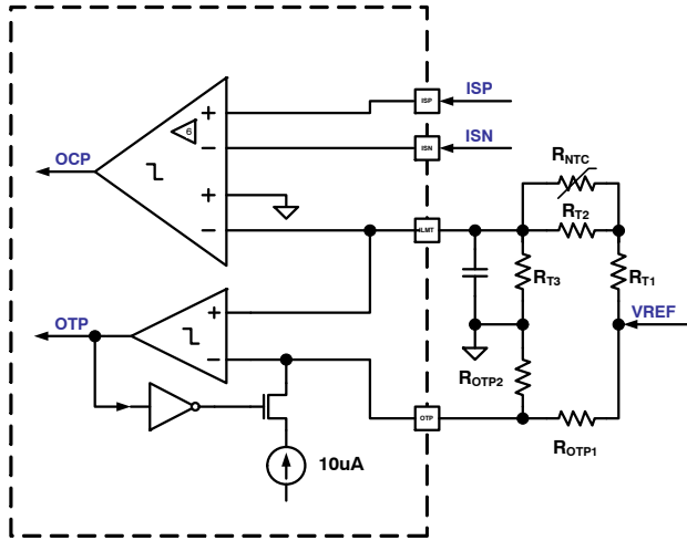
(1) OTP Configuration 1
