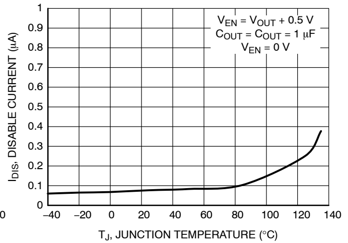
Figure 70. Disable Current vs. Temperature
