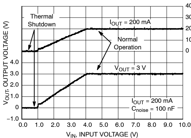
Figure 43. Thermal Shutdown Protection V_{OUT} = 3\ V , C_{noise} = 100\ nF , C_{OUT} = 1\ \mu F
