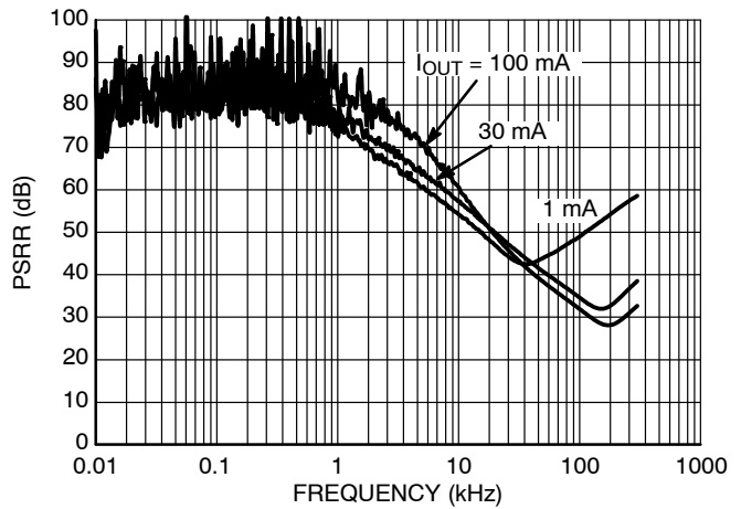
Figure 20. PSRR, 2.8 V Version, V_{IN} = 4.8\text{ V}
