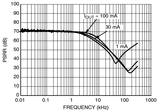
Figure 18. PSRR, 1.2 V Version, V_{IN} = 3.0\text{ V}
