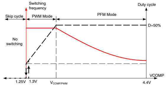
Figure 57. Mode Change with COMP Voltage
