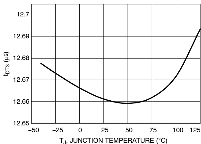
Figure 74. t DT3 vs. Temperature
