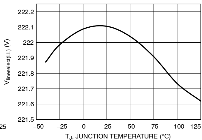
Figure 55. V lineselect(LL) (Version C5) vs. Temperature
