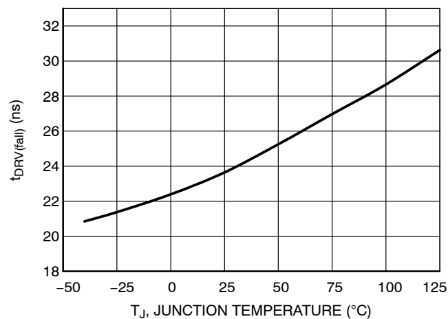
Figure 76. t DRV(fall) vs. Temperature
