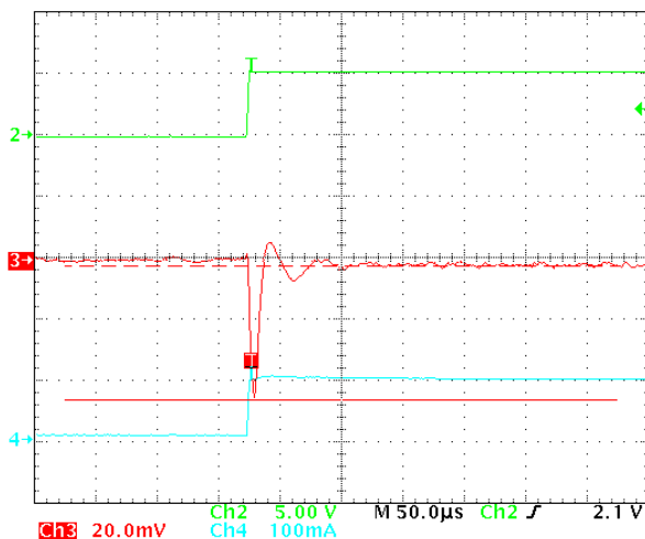
Figure 17. 10 mA to 100 mA Load Transient in 1\text{ }\mu\text{s} ( V_{IN} = 3.6\text{ V} , V_{OUT} = 1.2\text{ V} , Temperature = 25^\circ\text{C} )
