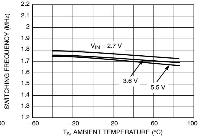
Figure 14. Switching Frequency vs. Ambient Temperature ( V_{out} = 1.2\text{ V} , I_{out} = 200\text{ mA} )
