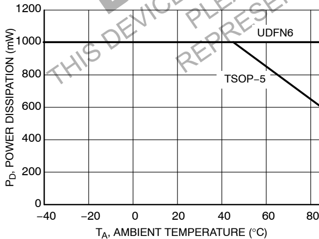
Figure 8. Power Derating
