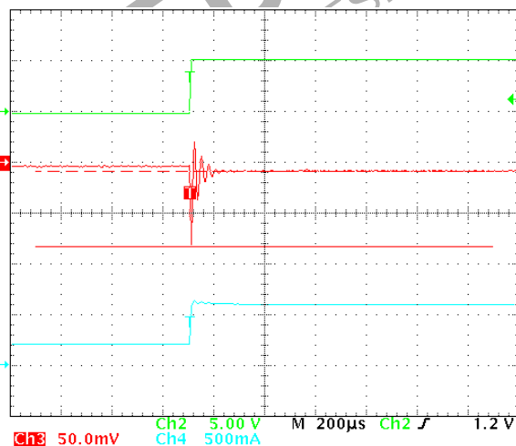
Figure 18. 200 mA to 600 mA Load Transient in 1\text{ }\mu\text{s} ( V_{IN} = 3.6\text{ V} , V_{OUT} = 1.2\text{ V} , Temperature = 25^\circ\text{C} )
