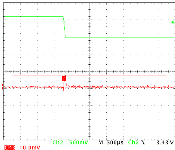
Figure 20. 3.6 V to 3.0 V Line Transient, Fall = 50\text{ }\mu\text{s} ( V_{IN} = 1.2\text{ V} , I_{OUT} = 100\text{ mA} , Temperature = 25^\circ\text{C} )
