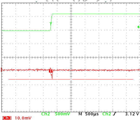
Figure 19. 3.0 V to 3.6 V Line Transient, Rise = 50\text{ }\mu\text{s} ( V_{IN} = 1.2\text{ V} , I_{OUT} = 100\text{ mA} , Temperature = 25^\circ\text{C} )
