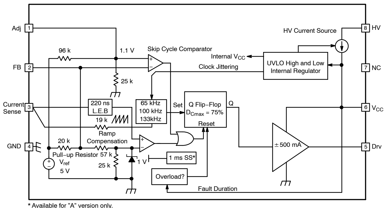
Figure 2. Internal Circuit Architecture
