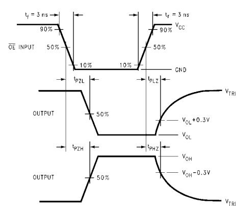
Figure 8. AC Waveforms
