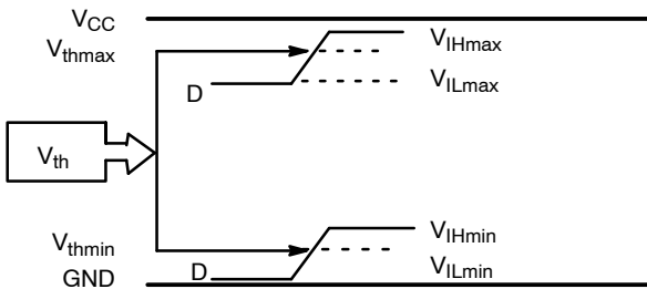
Figure 18. V_{th} Diagram
