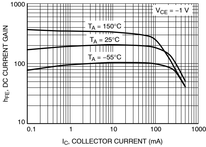
Figure 14. DC Current Gain vs. Collector Current
