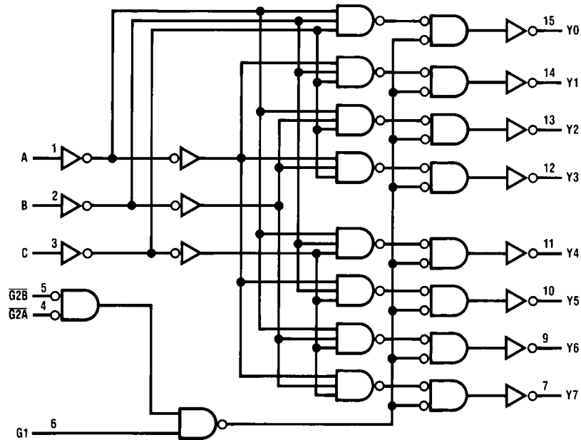
Figure 2. Logic Diagram
