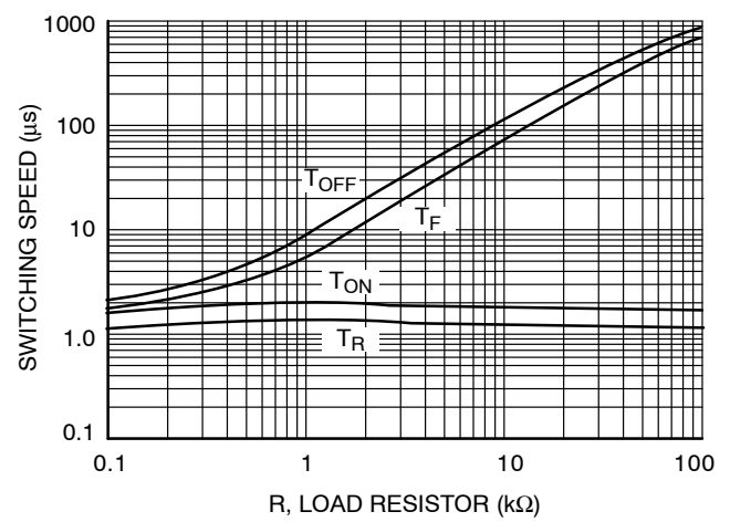
Figure 4. Switching Speed vs. Load Resistor
