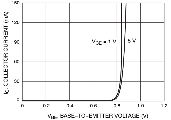
Figure 2. I_C - V_{BE}
