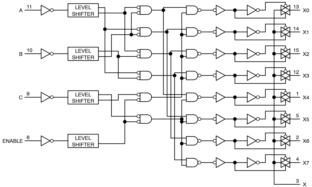
Figure 20. Function Diagram, 4051
