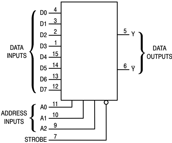
Figure 2. Logic Diagram
