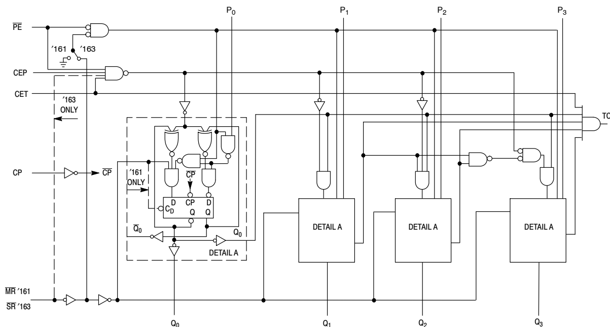
Figure 4. Logic Diagram
