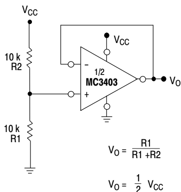
Figure 9. Voltage Reference
