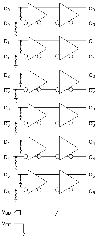
Figure 2. Logic Diagram
