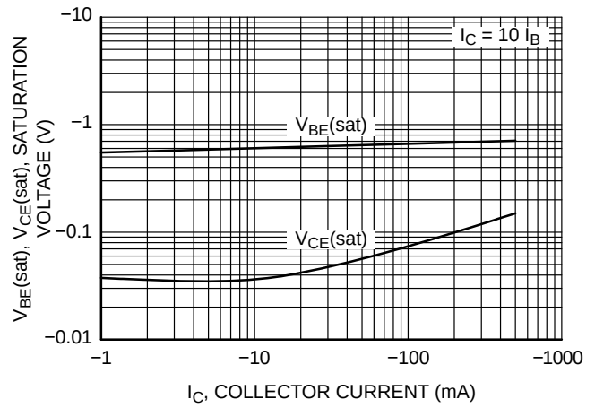
Figure 2. Collector-Emmitter Saturation Voltage and Base-Emmitter Saturation Voltage
