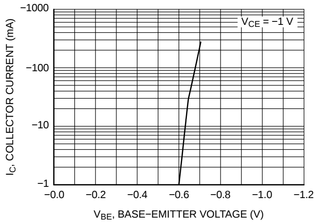
Figure 3. Base-Emmitter On Voltage
