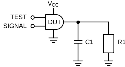
Figure 2. Test Circuit
