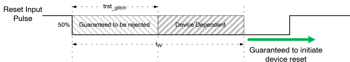
Figure 3. Reset Pulse Duration and Input Glitch Rejection Timing Diagram
