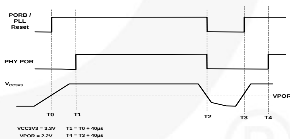
Figure 4. Power-On Reset Sequence
