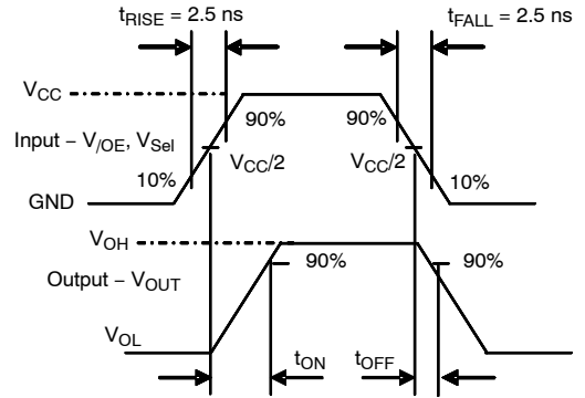
Figure 12. Turn-On / Turn-Off Waveforms
