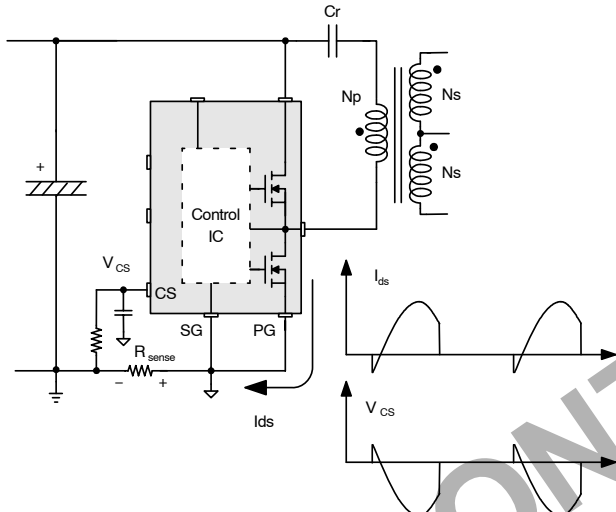
Figure 23. Half-Wave Sensing
