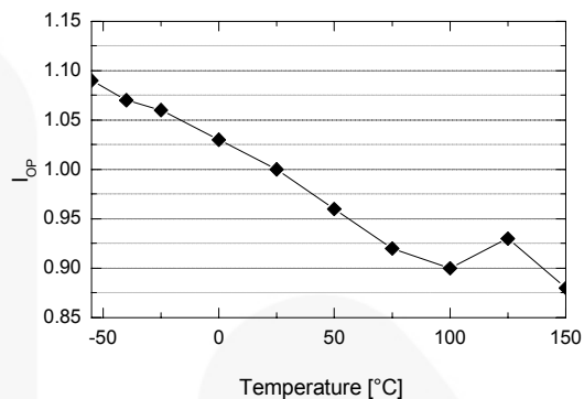
Figure 5. Operating Supply Current ( I_{OP} ) vs. T_A
