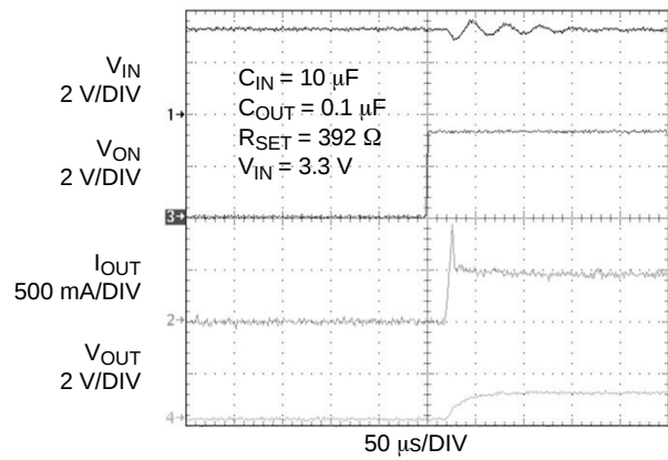
Figure 23. Current Limit Response Time (Output is Loaded by 2.2 \Omega , C_{OUT} = 10 \mu\text{F} )
