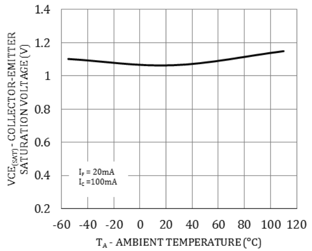
Figure 8. Collector Emitter Saturation Voltage vs. Ambient Temperature
