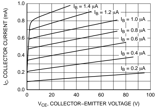
Figure 2. Static Characteristic
